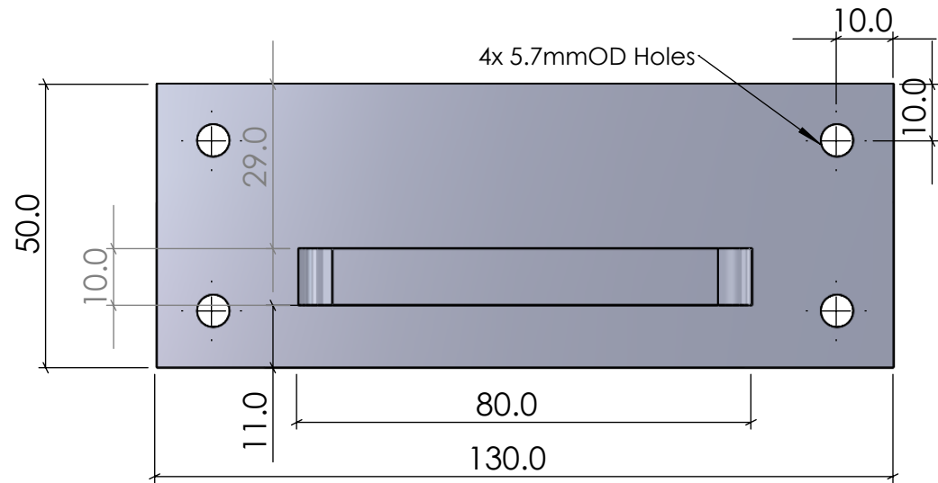
BOTTOM VIEW
